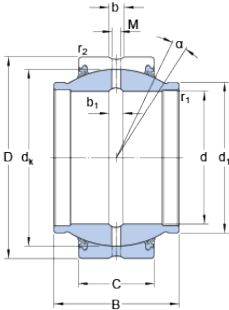
GEM 50 ES-2RS Bearing 2D drawings and 3D CAD models
